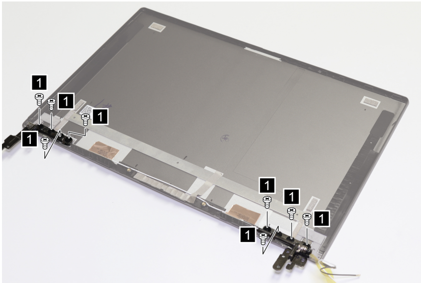
Figure 39. Remove eight screws
