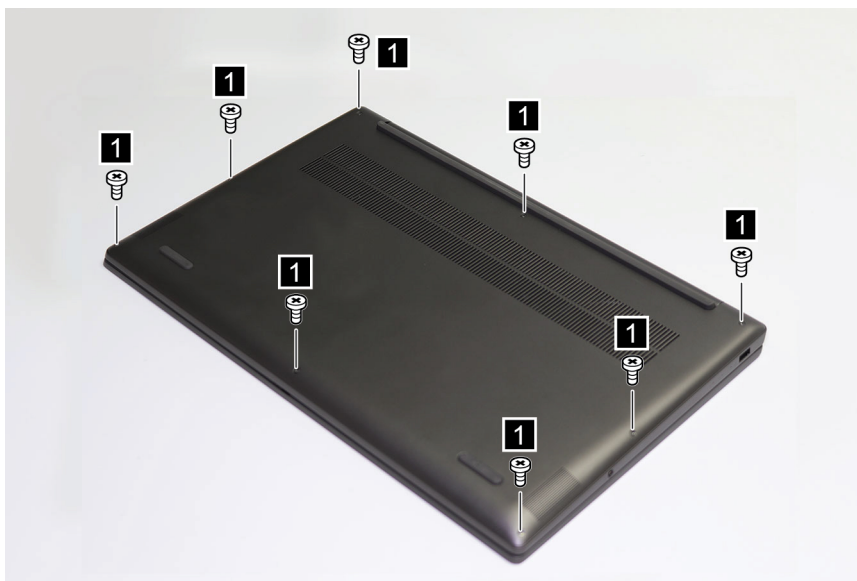
Figure 2. Remove eight screws
