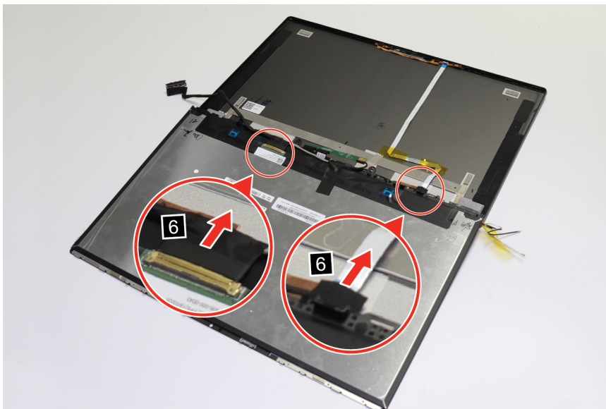
Figure 31. Disconnect the cables from the LCD panel
