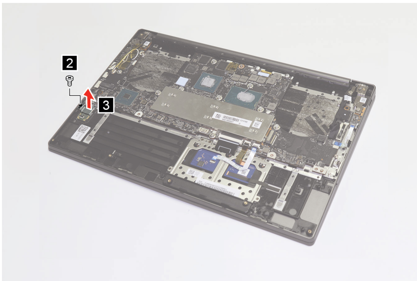
Figure 19. Remove one screw and the fingerprint bracket
