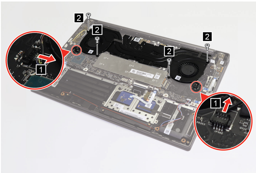
Figure 10. Disconnect the thermal module cable connectors and remove four screws
