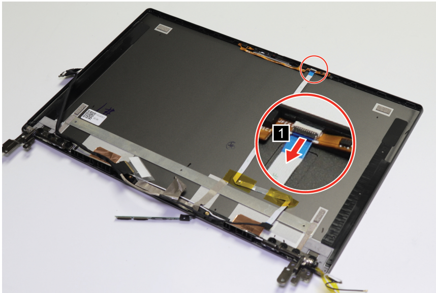
Figure 36. Disconnect the camera connector
