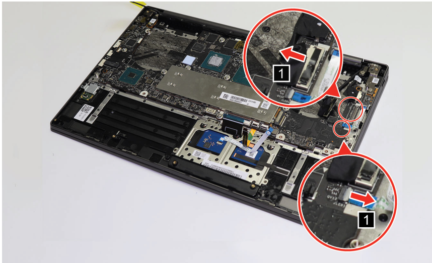
Figure 22. Disconnect the LED FPC and EDP cable from the system board
