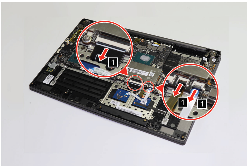
Figure 21. Disconnect the keyboard FPC and touchpad FPC
