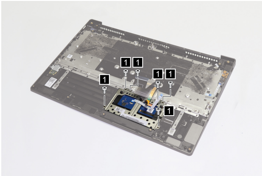
Figure 26. Remove six screws
