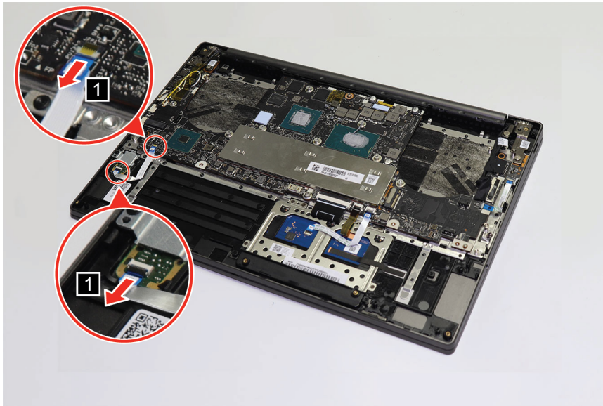
Figure 18. Disconnect the fingerprint module connectors
