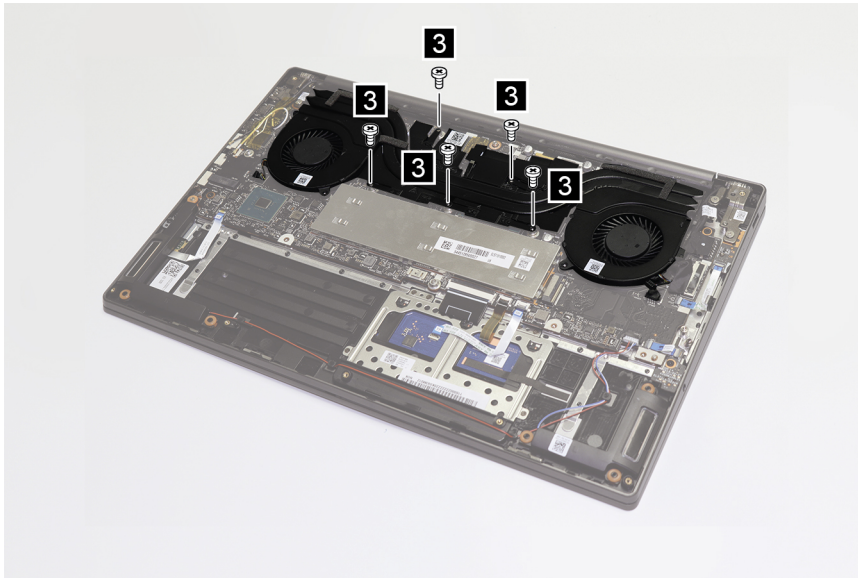
Figure 11. Remove five screws
