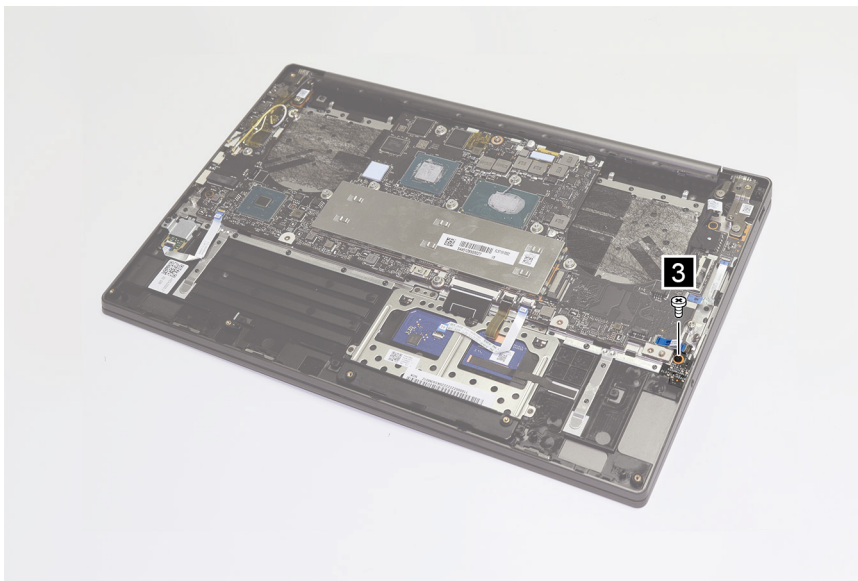
Figure 16. Remove one screw
