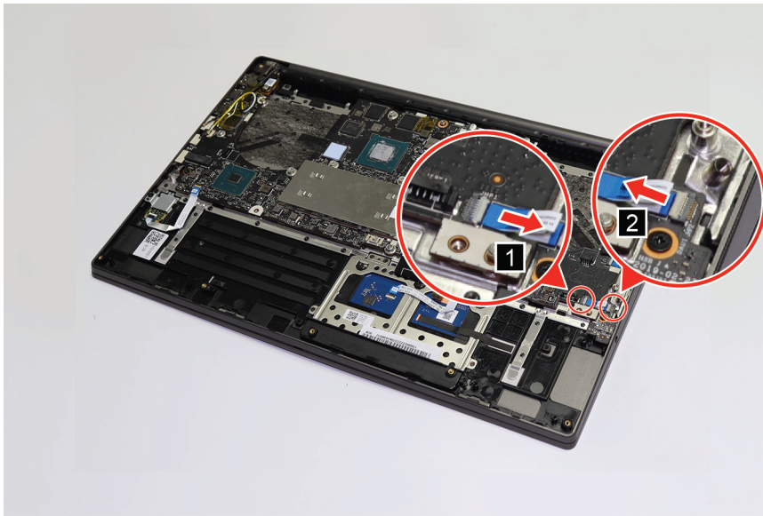
Figure 15. Disconnect the audio board connectors
