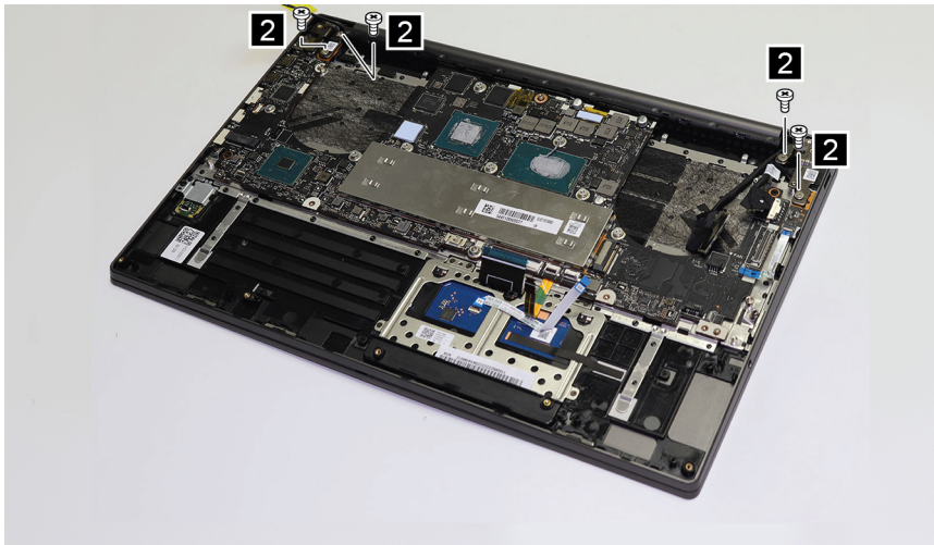
Figure 23. Remove four screws
