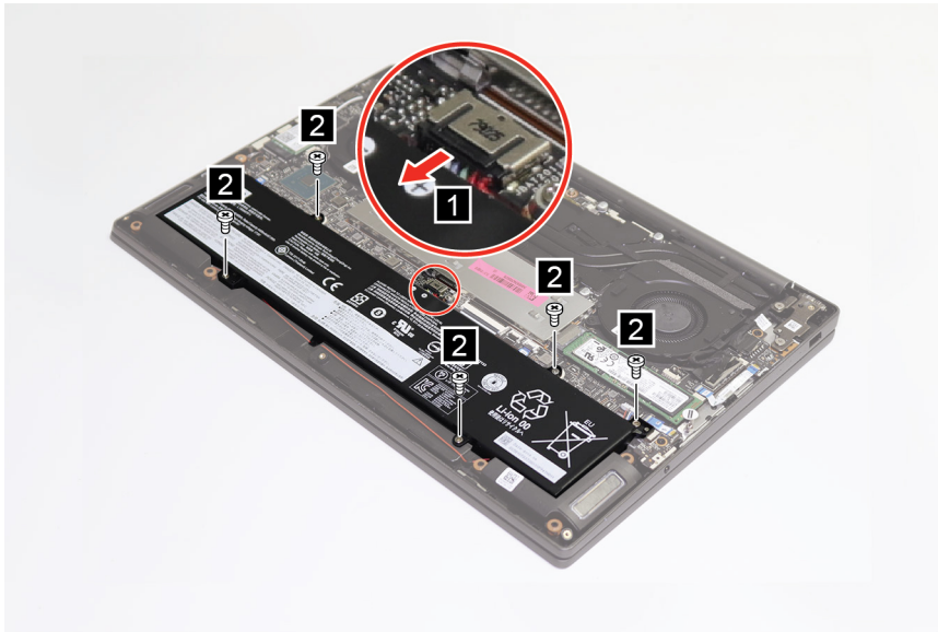
Figure 4. Disconnect the cable and remove five screws.
