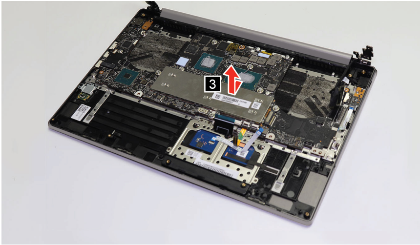
Figure 24. Remove the upper case
