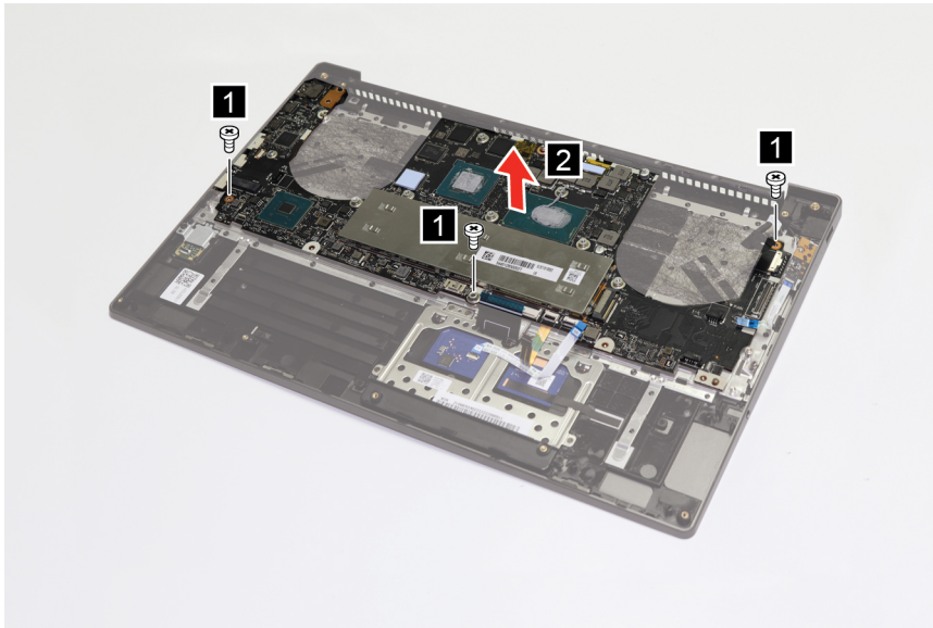
Figure 25. Remove three screws and the system board
