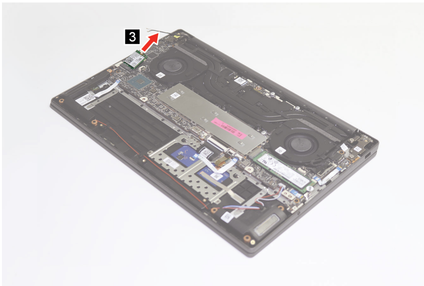
Figure 7. Pull the WLAN card out of the slot
