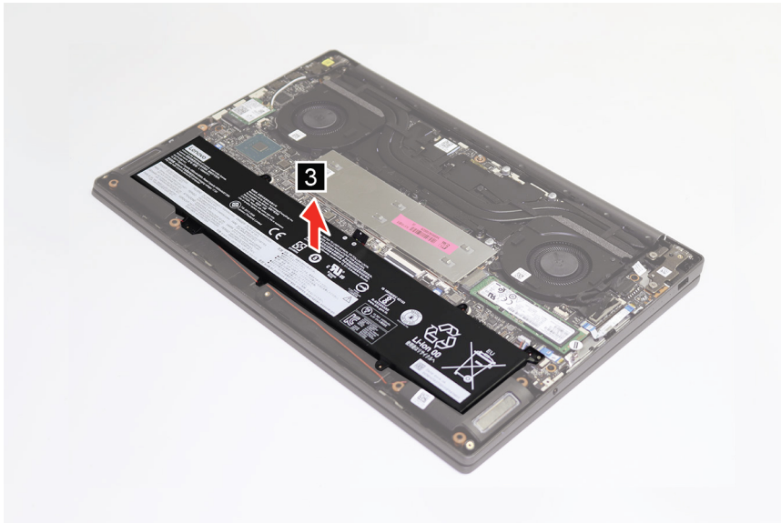
Figure 5. Remove the battery pack
