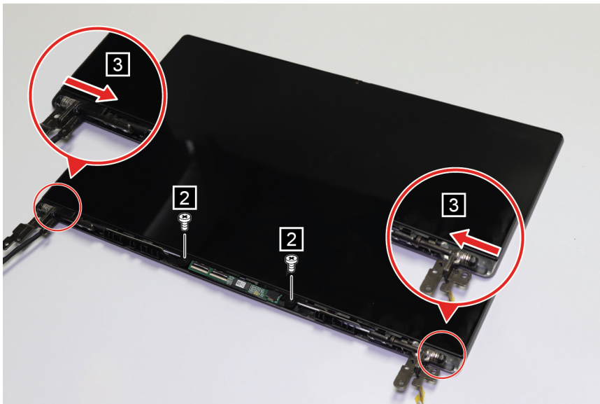
Figure 29. Remove two screws and strip covers
