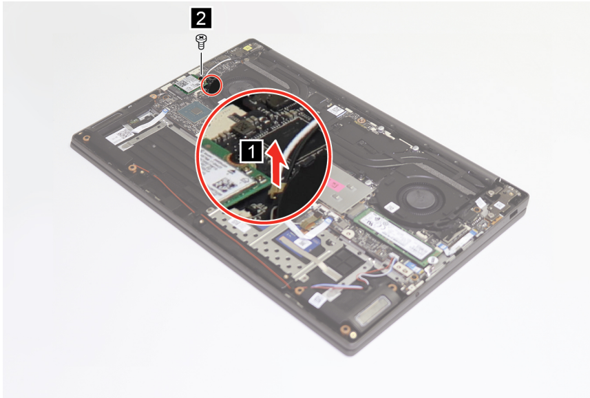
Figure 6. Disconnect the wireless antenna cables and remove one screw
