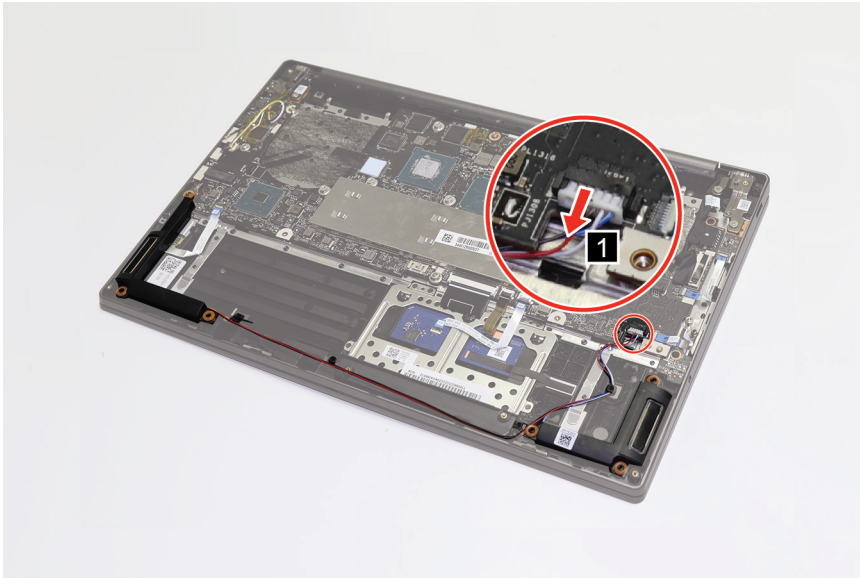
Figure 13. Disconnect the cable and release the cables from hooks
