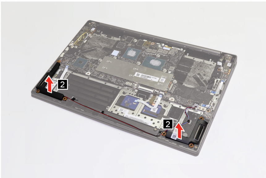
Figure 14. Remove the speakers
