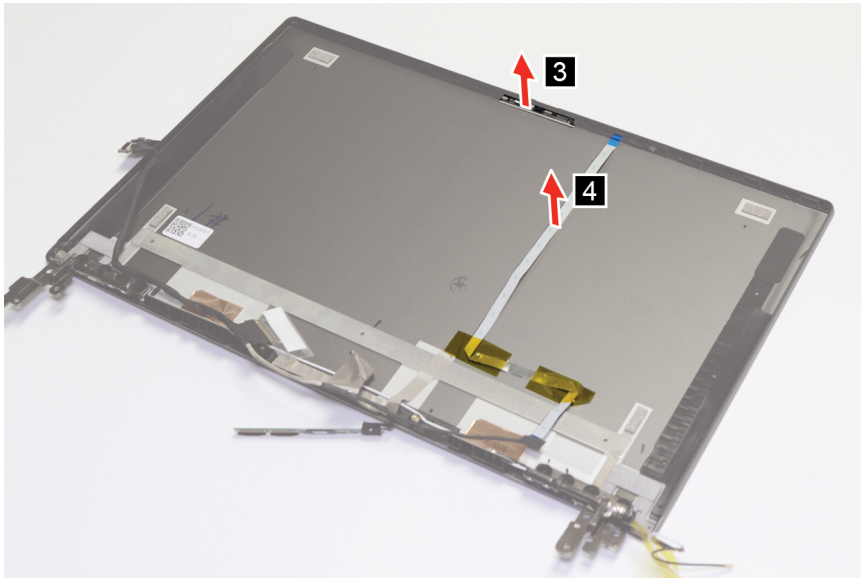
Figure 38. Remove the camera module and the LED FPC
