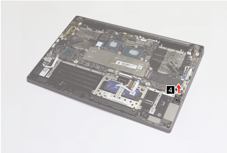
Figure 17. Remove the audio board
