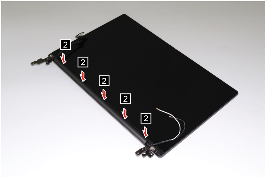
Figure 35. Press down on the hinge cap
