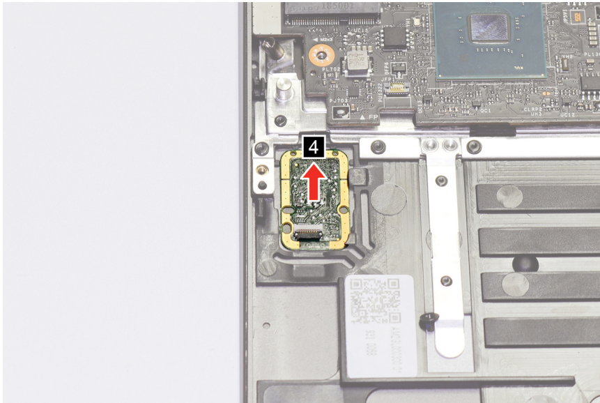
Figure 20. Remove the fingerprint module
