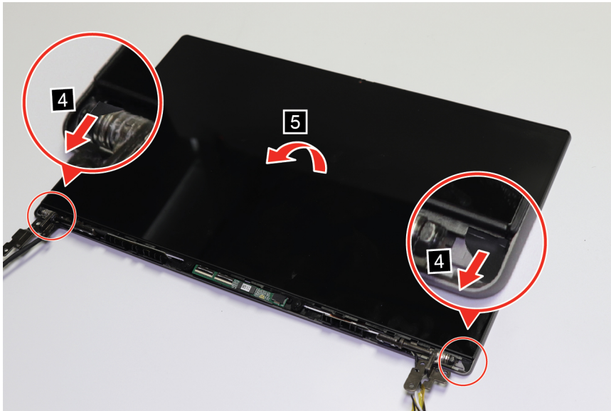
Figure 30. Pull out the LCD panel adhesive and turn the LCD panel
