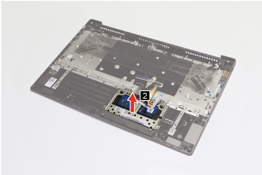
Figure 27. Remove the touchpad with cable
