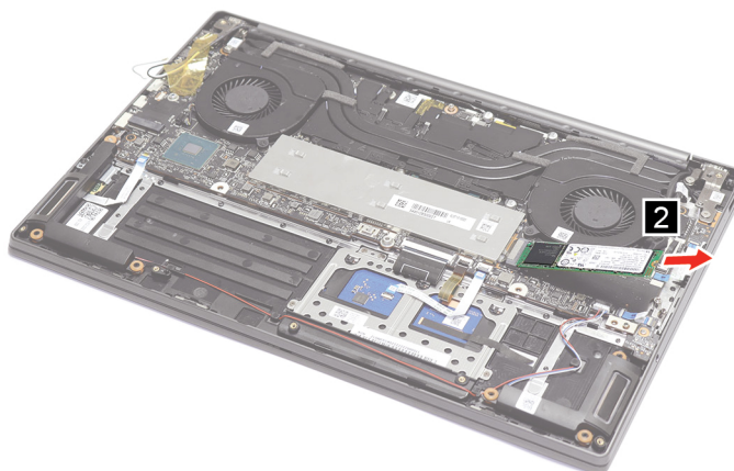
Figure 9. Pull the solid-state drive out of the slot
