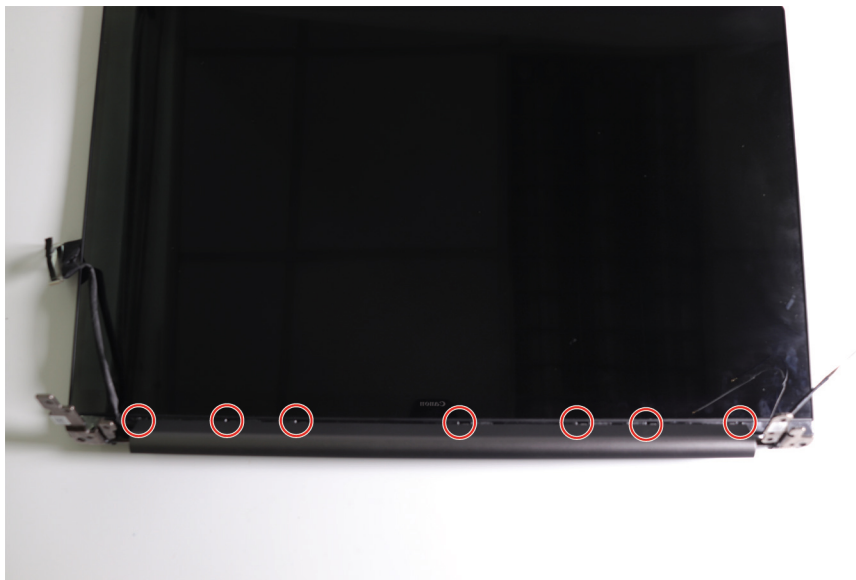
Figure 33. Press down on the hinge cap
